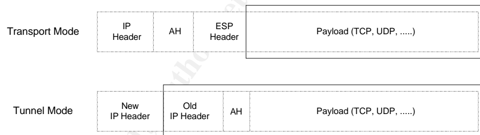
Figure 7. ESP Encapsulation
