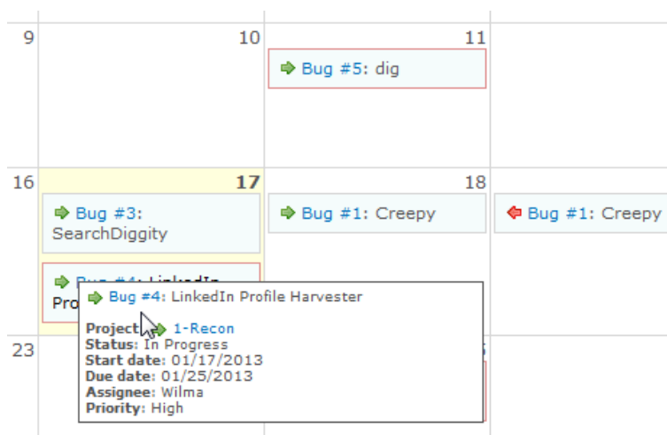
Figure 11: Redmine calendar
