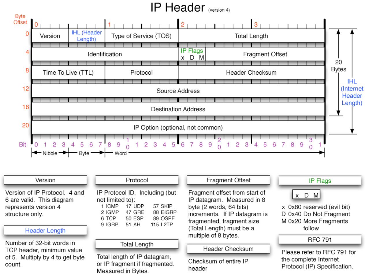
Figure 7.3: IP Header
